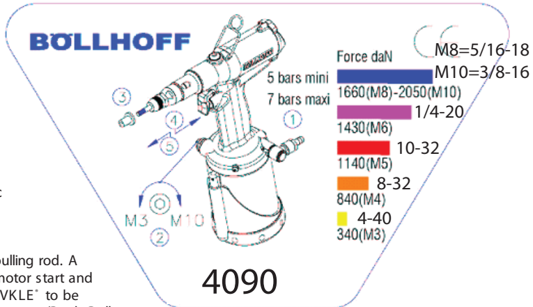
Figure 11 - Adjustment Guide
