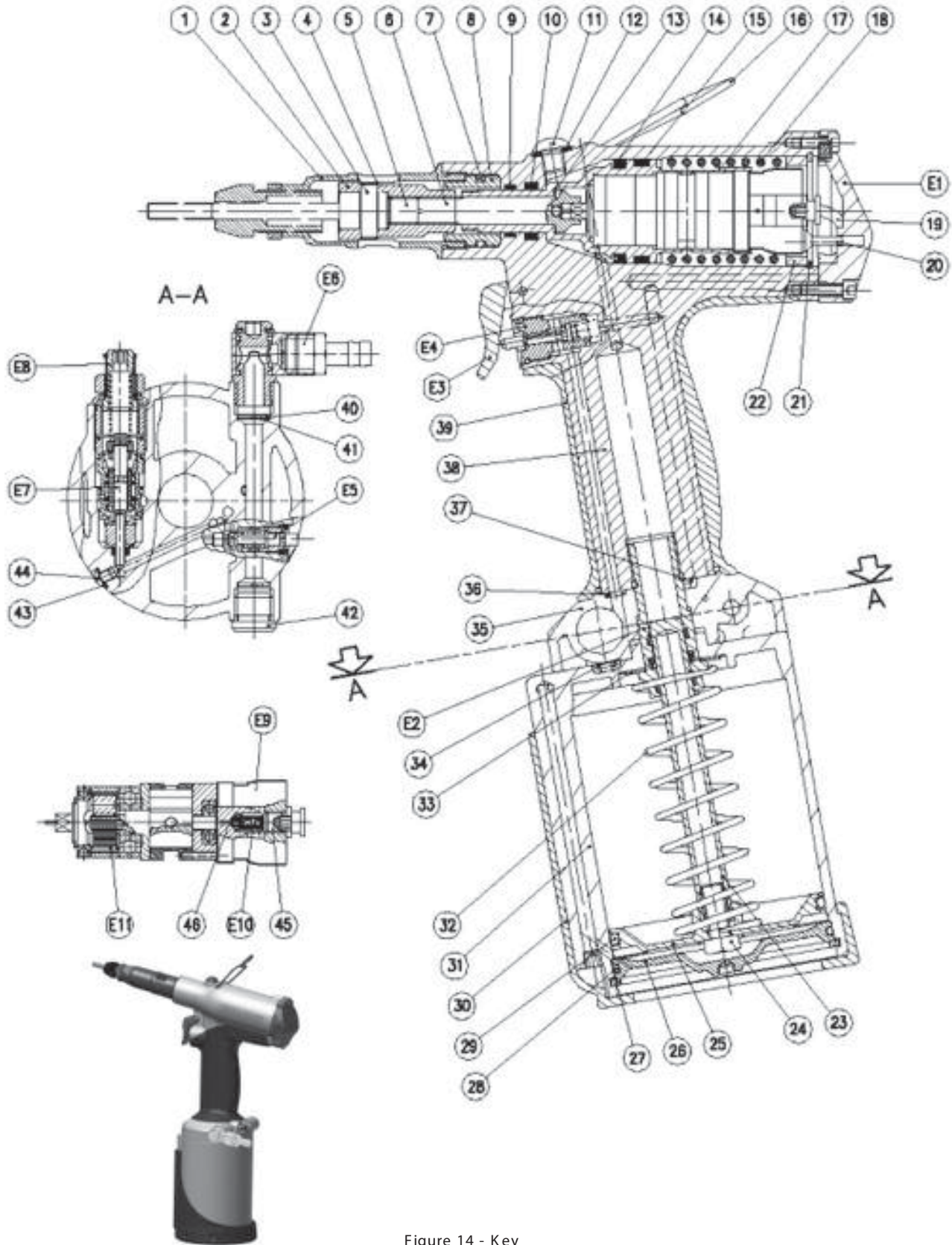
Figure 14 - Key
