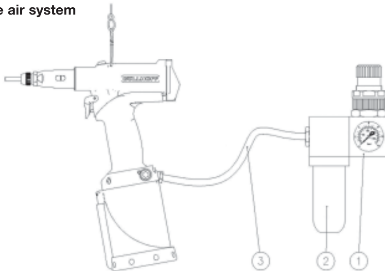
Figure 10 – Air connection
