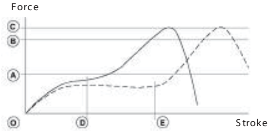
Figure 3 - Force/stroke graph
