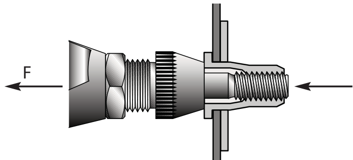
Figure 2 - Pressure setting principle
