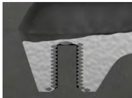
The liquid melted aluminium fills the mould and encloses the IMTEC® CO without flowing into the internal thread.
