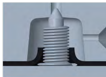
Mould closing
